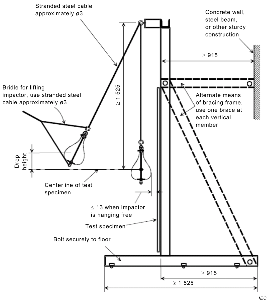
Figure 6 – Impact test frame 1
